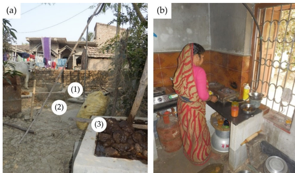
Figure 7. Household biodigester (a) Deenbandhu Model: (1) inlet filled with manure and water; (2) underground fixed-dome fermenter, and (3) outlet chamber in the rural village of Ghoragachha, West Bengal India. (b). Women cooking on a biogas stove, directly connected with the biodigester.
